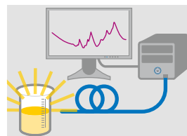
Optical spectroscopy
